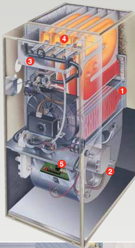
Model 355BAV
